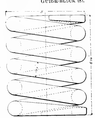
Fig. 4700. TRUCK BOLSTER SPRING. Standard Coil.
